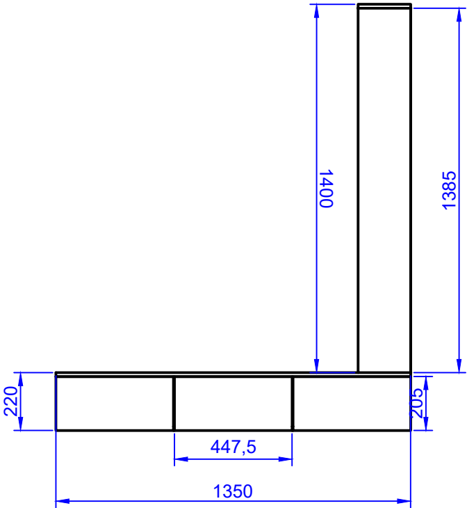
VISTA FRONTAL
