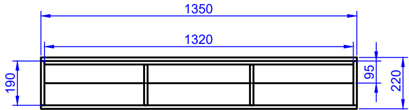
VISTA FRONTAL
